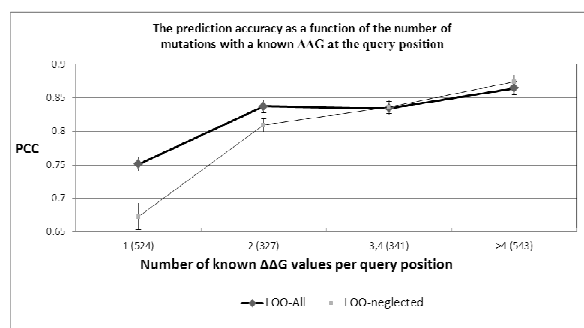
Figure 2. The PCC of Pro-Maya on the PoPMuSiC-DB vs. the number of known mutations at the query position using the LOO-all and LOO-neglect. The number of mutations in each group is shown in parentheses. For example, the second data point of the black curve indicates the performance of Pro-Maya on 327 query mutations with two known records for each in the training set. The second data point of the grey curve indicates the performance of Pro-Maya on the same subset of mutation after one of the two known mutations was removed from the training set. The first data point of the grey curve was calculated using the \Delta\Delta G^{RF} . The difference between the grey and black curves indicates the PCC improvement achieved by the addition of a single known mutation in the query position. The results suggest that the improvement in accuracy is facilitated by the incorporation of as few as 1-2 known \Delta\Delta G values in the query position.
