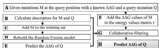
Figure 1. Prediction scheme for a query mutation with known \Delta\Delta G values for additional mutations at the same position. (A) The input for this prediction scheme includes query (Q) and known (M) mutations at the query position. The \Delta\Delta G value for M is known. (B-E) Calculate the predicted \Delta\Delta G of Q using the Random Forests algorithm. (F) Add the \Delta\Delta G values of M to the appropriate elements in the energy matrix r , according to the MU identity and position of M. (G) Given the training set (matrix r ), and the features (including the \Delta\Delta G predicted by Random Forests) start the stochastic gradient descent and calculate the \Delta\Delta G of Q (H).
